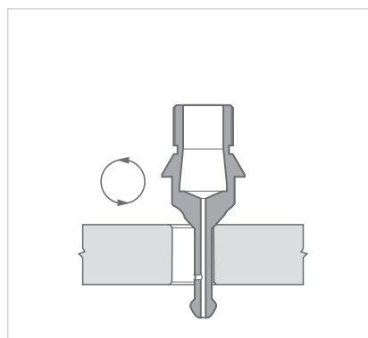
4_Upper countersinking
